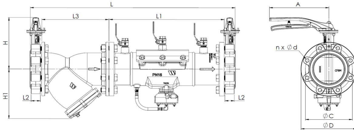
RPZ Butterfly Valve with Lever Handle
