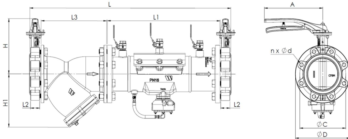
RPZ Butterfly Valve with Lever Handle
