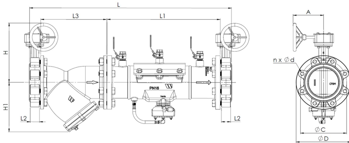
RPZ Butterfly Valve with Gearbox
